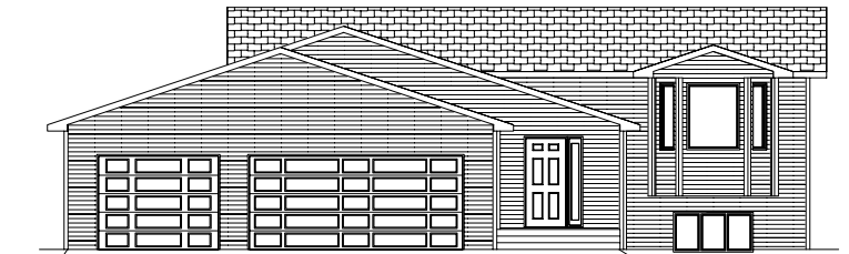
FRONT ELEVATION C
