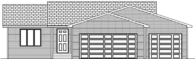
FRONT ELEVATION A
